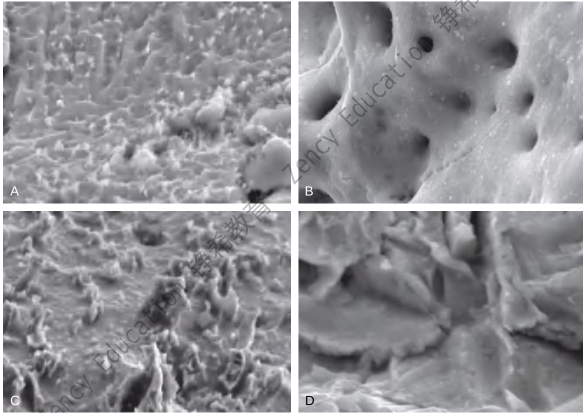
Figure 16-4 Modern implants display clear nanopatterns in contrast to their respective predecessors. A , Astra Tech OsseoSpeed implant. B , Nobel Biocare TiUnite implant. C , A Biomet 3i Nanotite implant. D , An example of a predecessor implant Astra TiOblast without the typical nanopattern. All images 50,000 \times or more in magnification.
