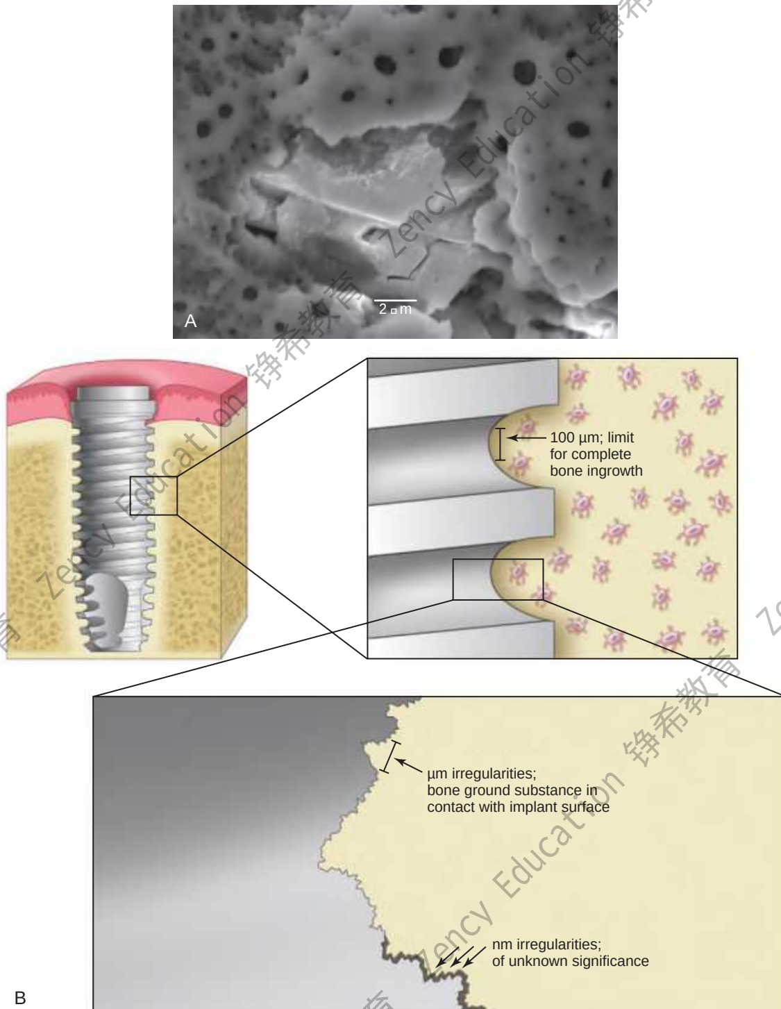
Figure 16-1 A , A moderately rough surface characterized by an S_a of 1 to 2 \mu\text{m} and an S_{dr}\% of 25 to 75 may serve as an example of most commercially available modern implants. This image presents a moderately rough blasted and anodized surface, with typical porosity achieved by anodisation. B , Bone tissue including ground substance and cellular components will need pores of a minimal size of 100 \mu\text{m} for ingrowth. Calcified ground substance of bone responds differently to irregularities in the micrometer size that are important for the strength of the osseointegrated response. Implant irregularities in the micrometer range are, to date, of undetermined significance for osseointegration.
